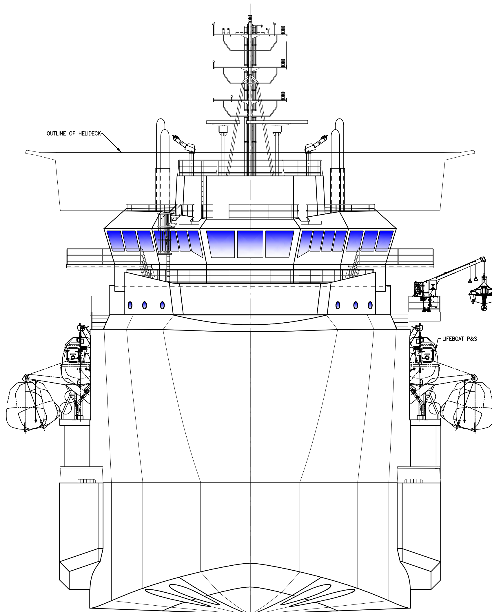
BOW LOOKING AFT
