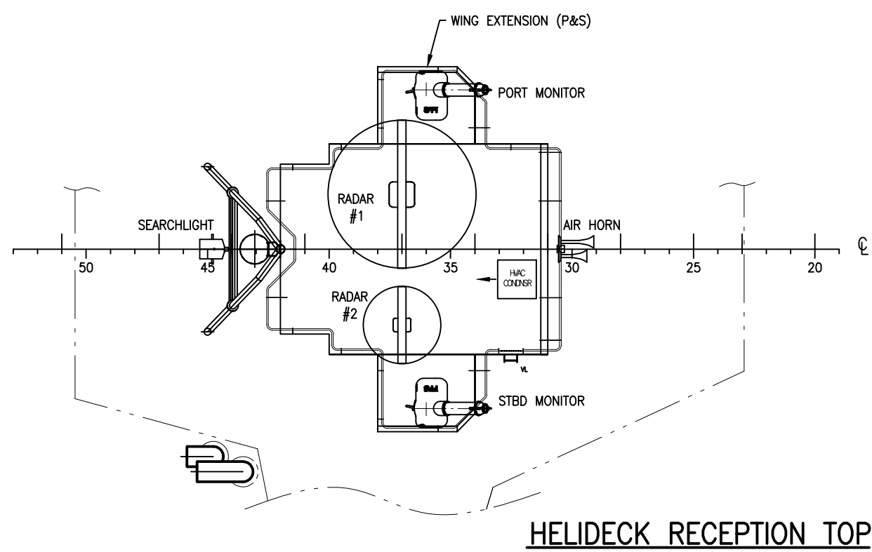
HELIDECK RECEPTION TOP
