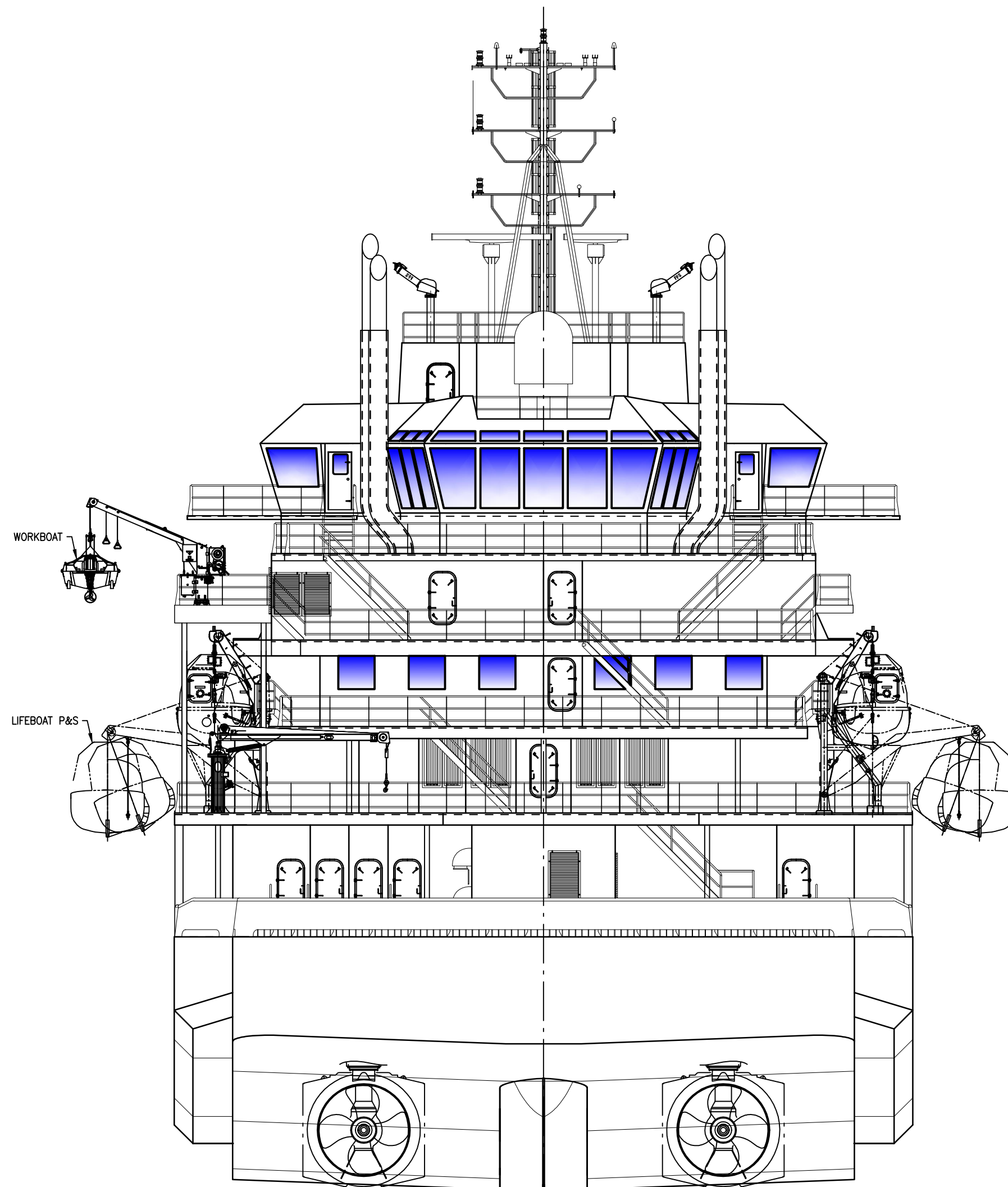
STERN LOOKING FWD DECK CRANE OMITTED FOR CLARITY
