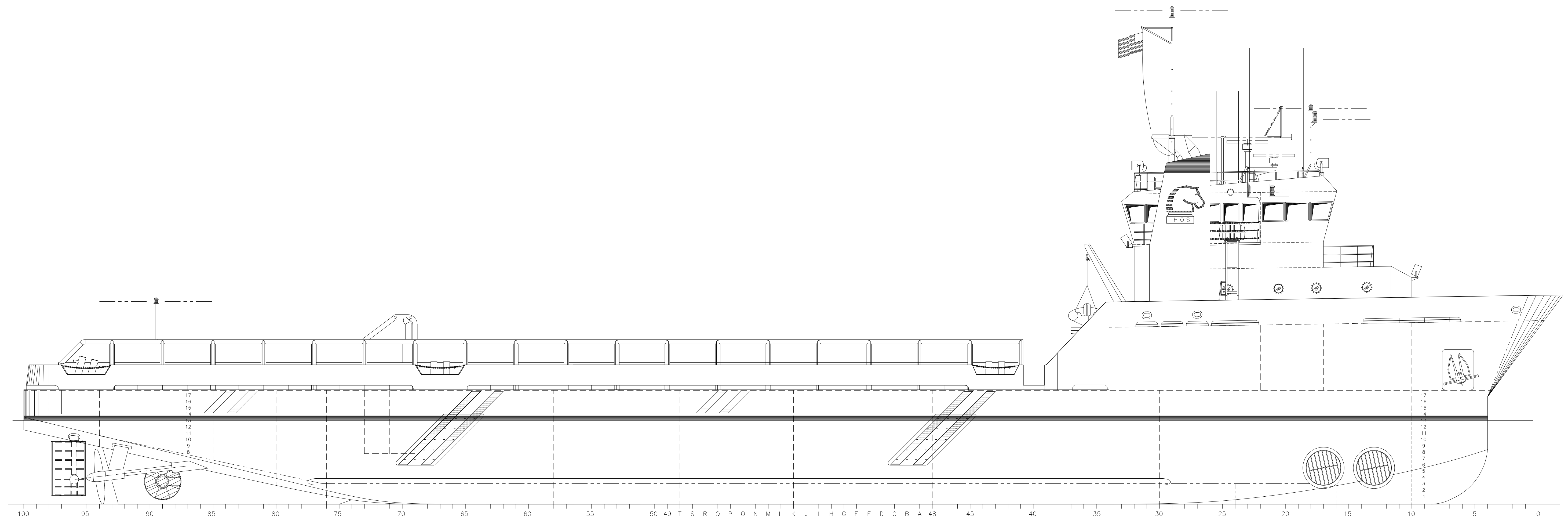
OUTBOARD PROFILE
