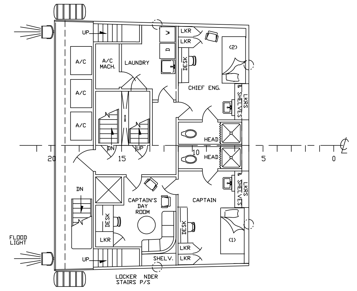
01 LEVEL 35'-0" ABOVE BASELINE
