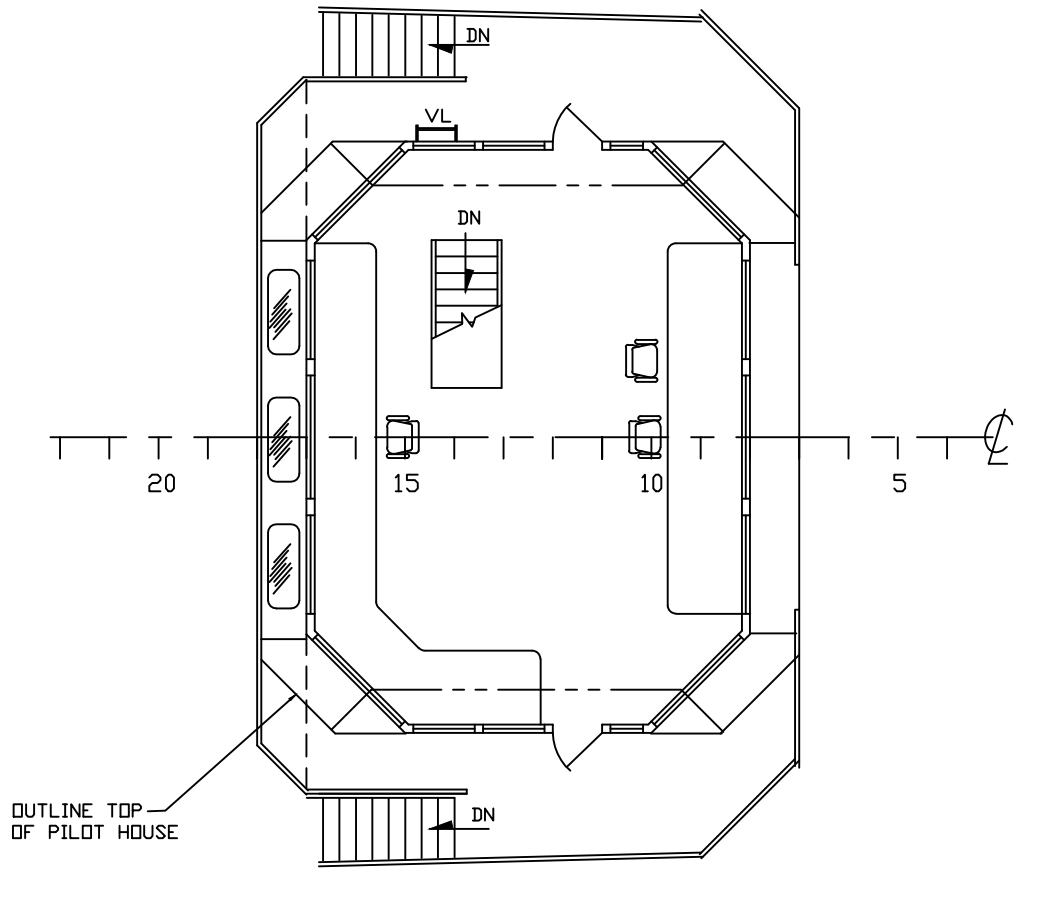
BRIDGE 44'-0" ABOVE BASELINE
