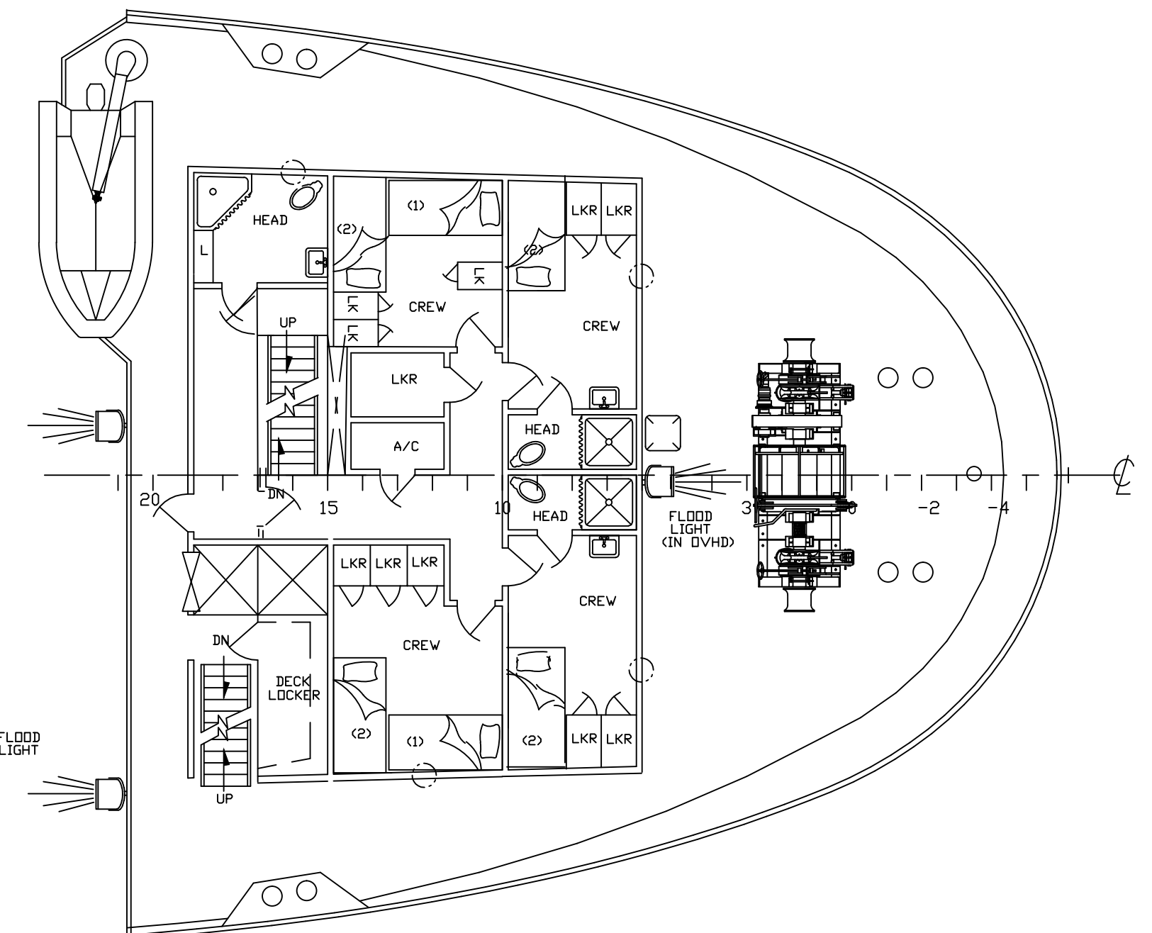
FOCSLE DECK (26'-0" ABOVE BASELINE)
