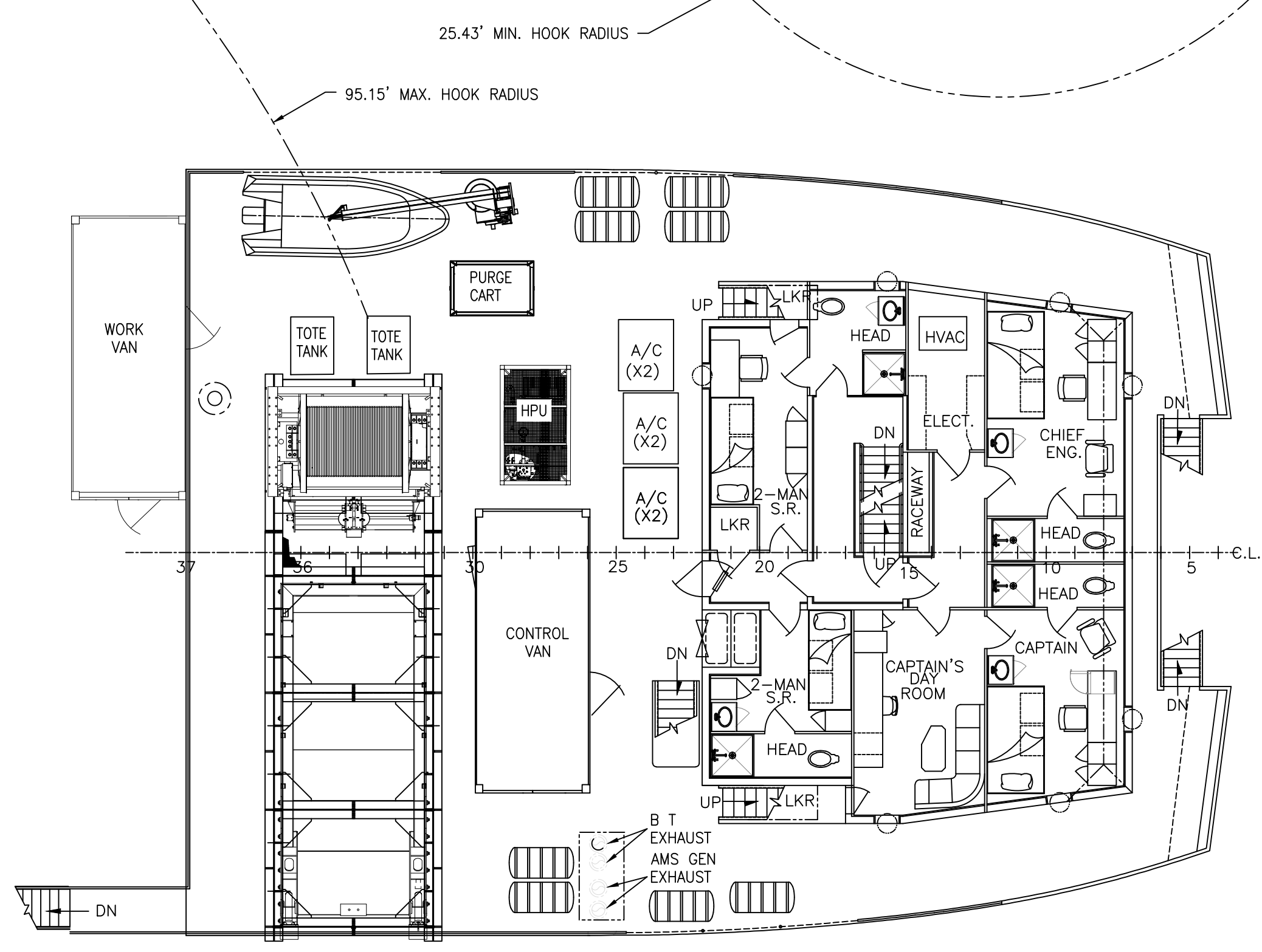
PLAN AT 01 LEVEL @ 37'-6" ABV. BASELINE SCALE: 1/8" = 1'-0"
