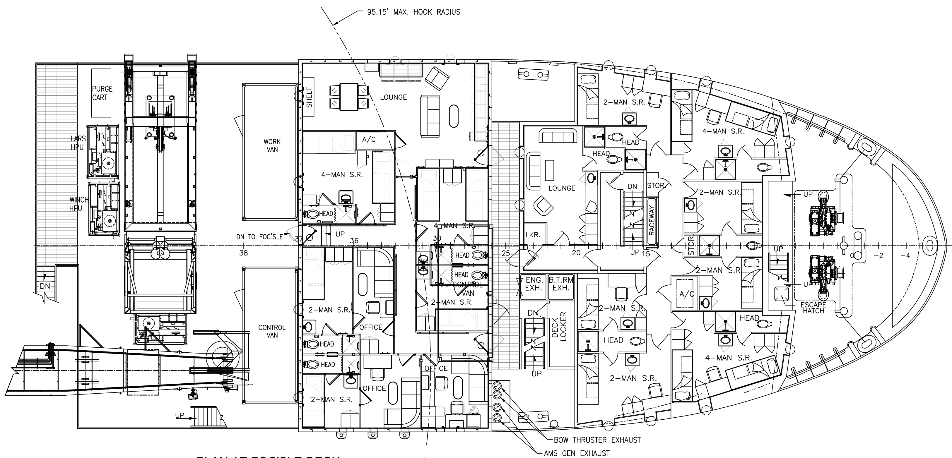
PLAN AT FOC'SLE DECK @ 28'-0" ABV. BASELINE SCALE: 1/8" = 1'-0"
