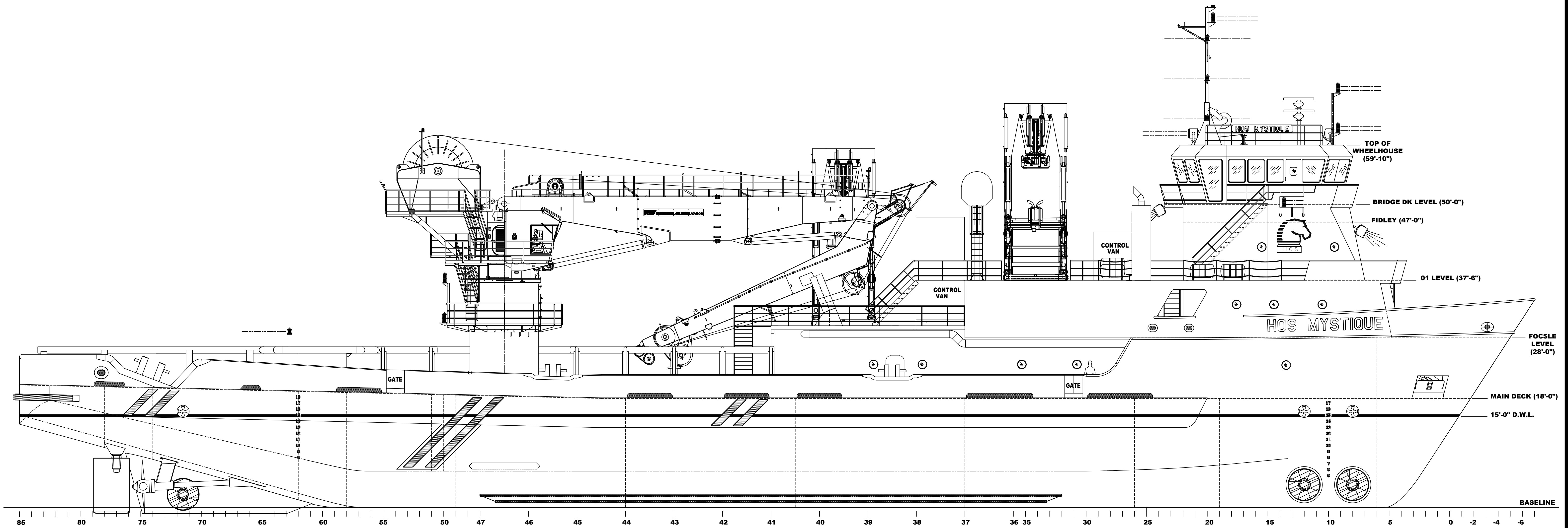
STBD SIDE PROFILE SCALE: 1/8" = 1'-0"
