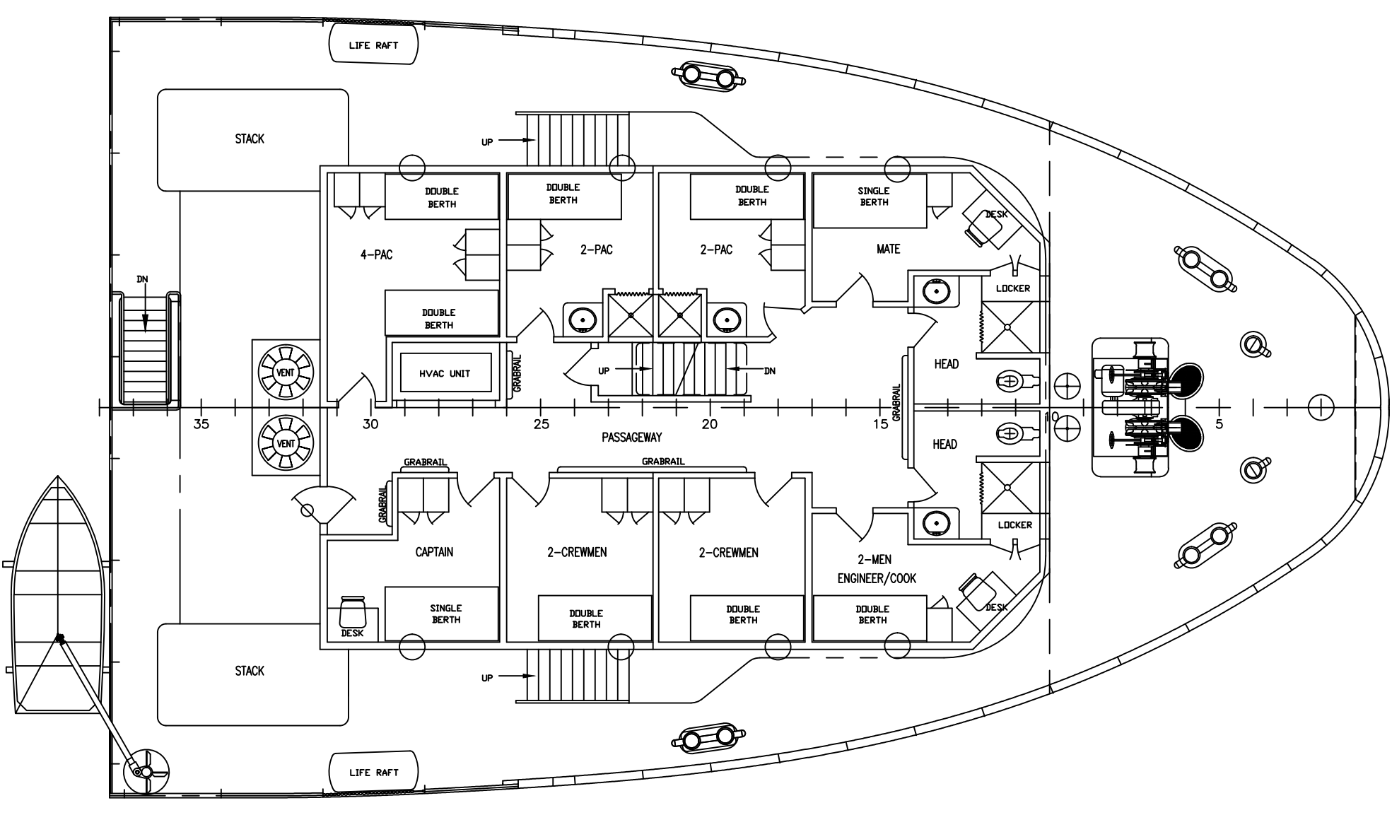
FDC'SLE DECK 27'-9" ABOVE BASELINE
