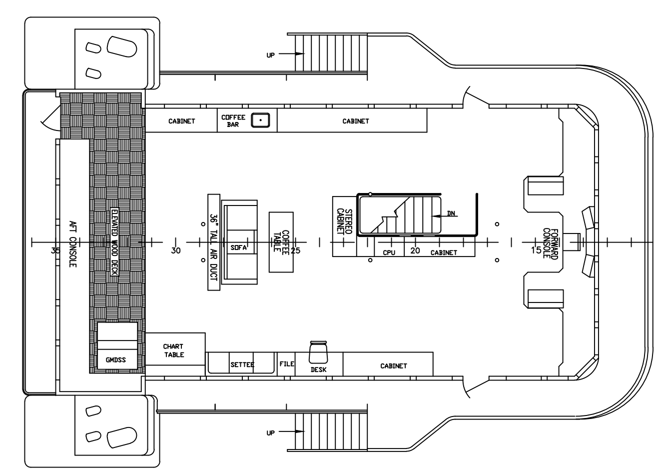
BRIDGE DK LEVEL 36'-6" ABOVE BASELINE
