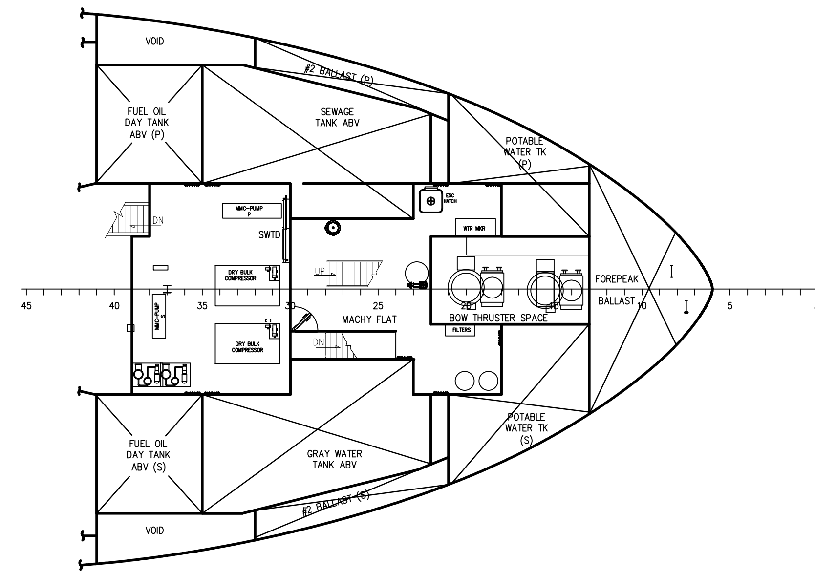
MEZZANINE FLAT
