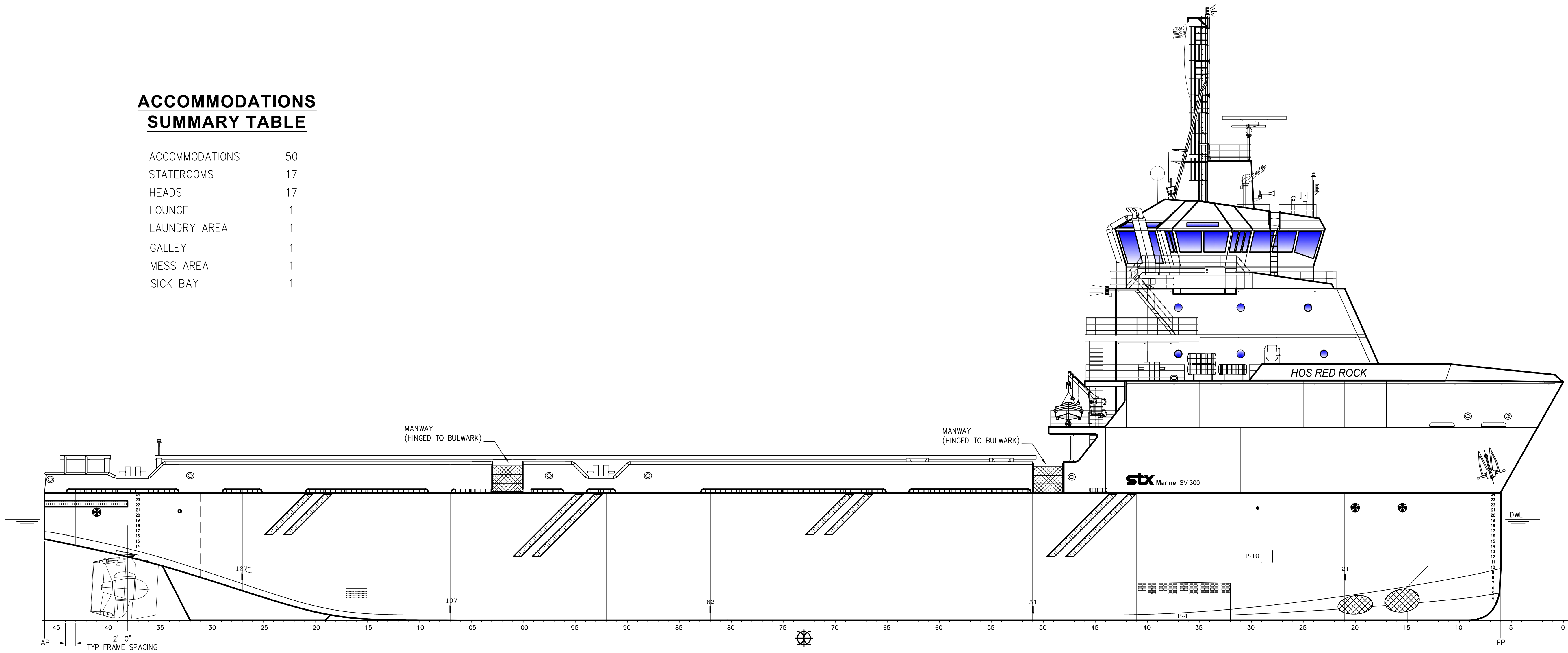
OUTBOARD PROFILE
