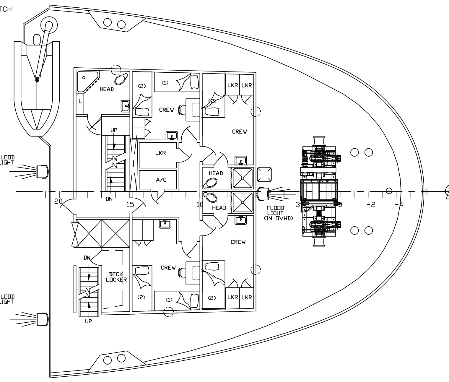
FOCSLE DECK (26'-0" ABOVE BASELINE)
