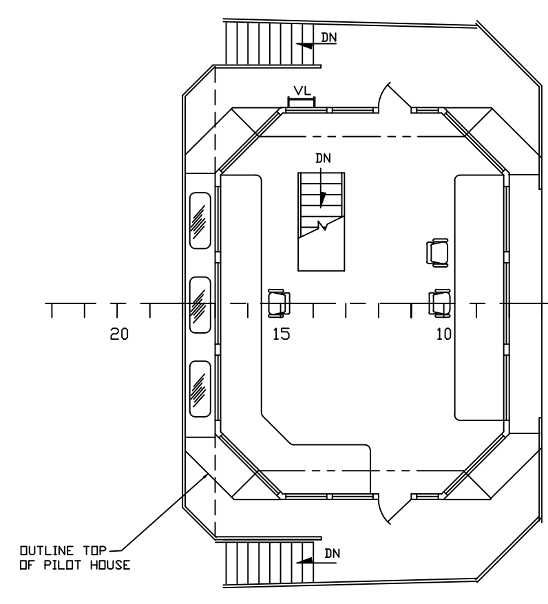
BRIDGE 44'-0" ABOVE BASELINE
