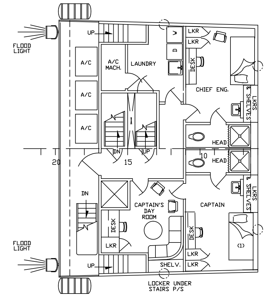
01 LEVEL 35'-0" ABOVE BASELINE
