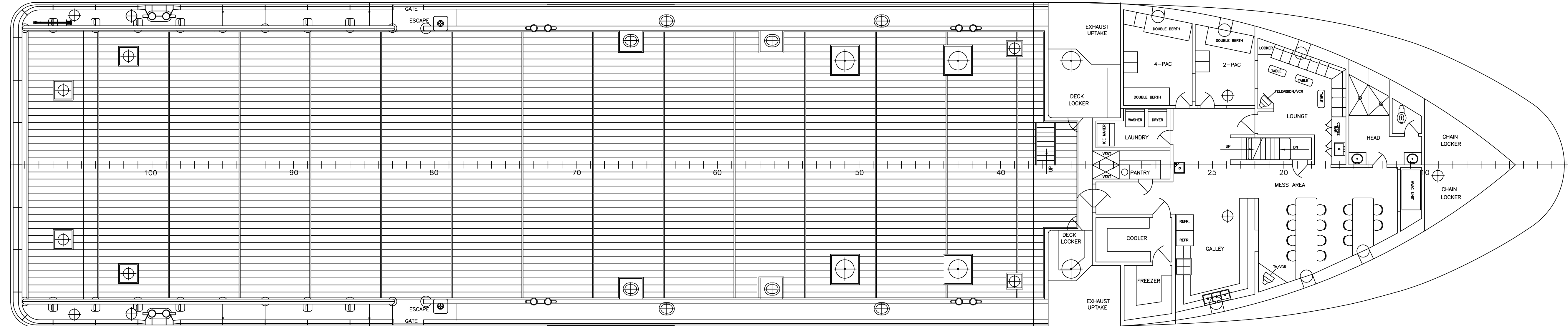
MAIN DECK 16'-0" ABOVE BASELINE
