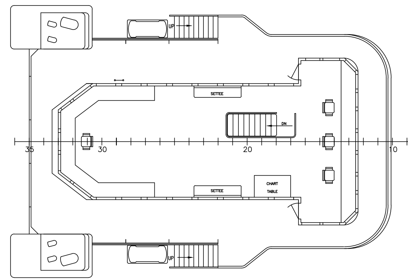
BRIDGE DK LEVEL 36'-6" ABOVE BASELINE
