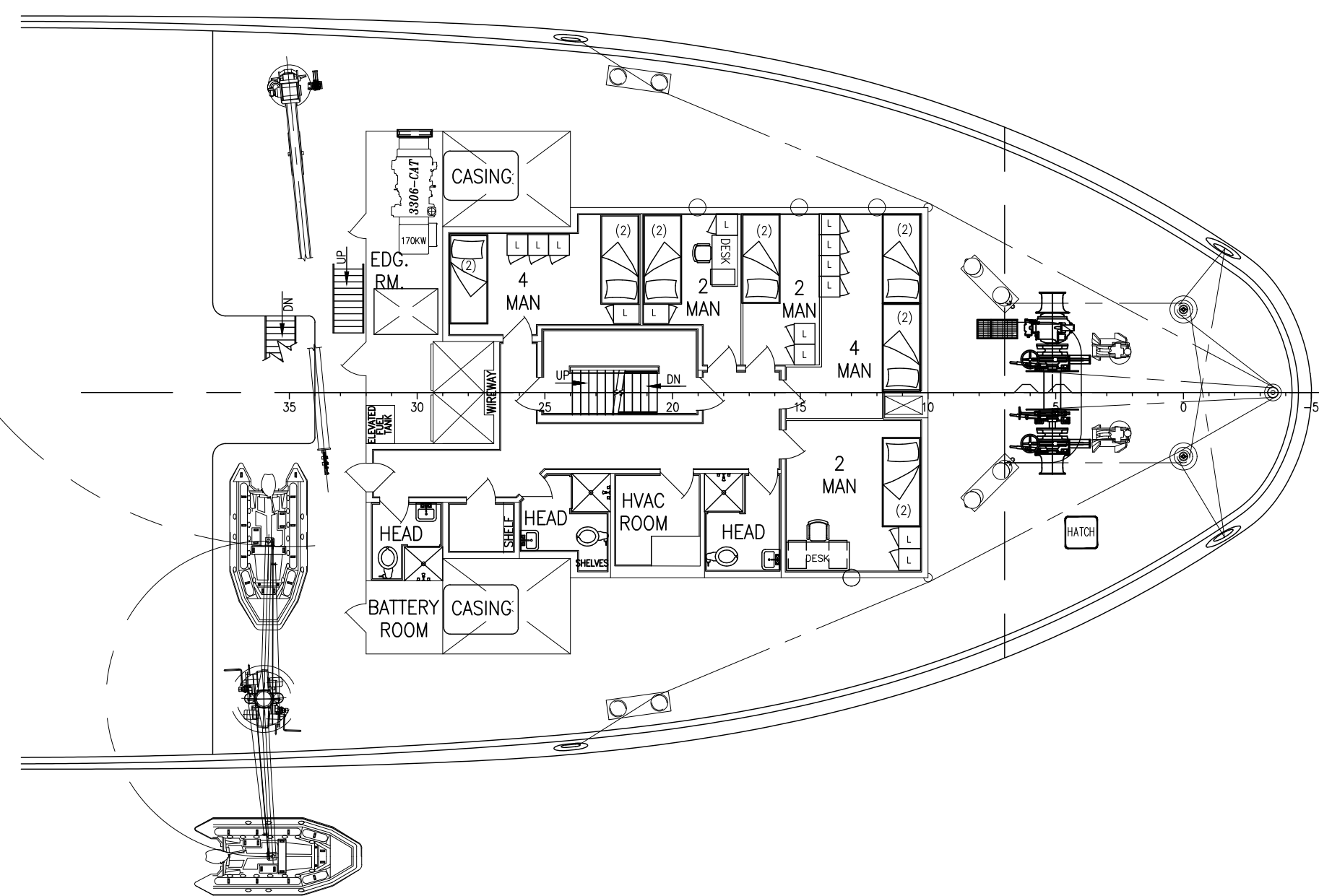
01 DECK PLAN 34'-2" ABL
