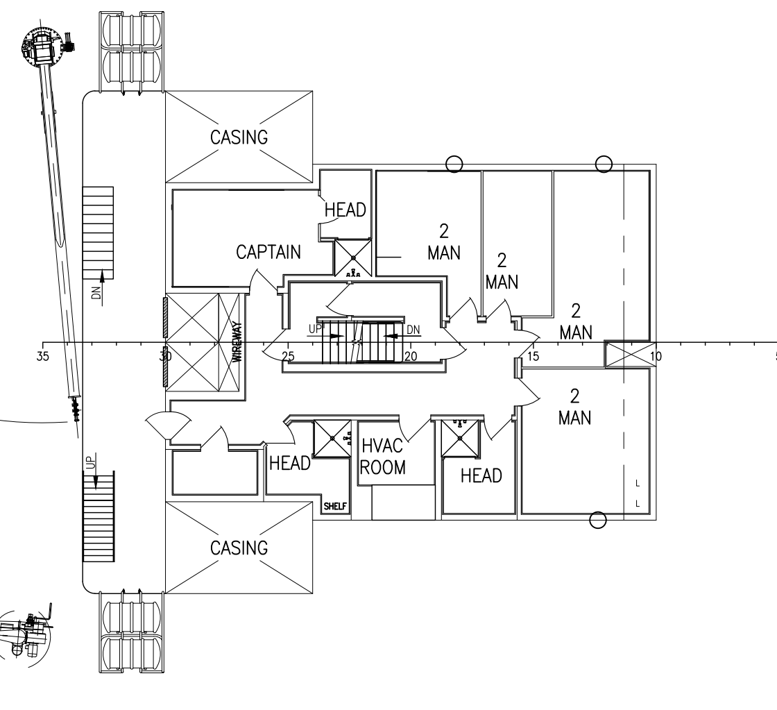
02 DECK PLAN 42'-6" ABL
