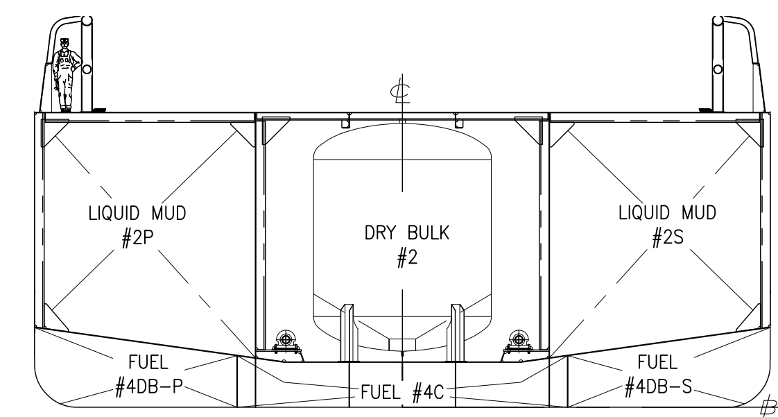
CARGO SECTION FR70 LKG FWD
